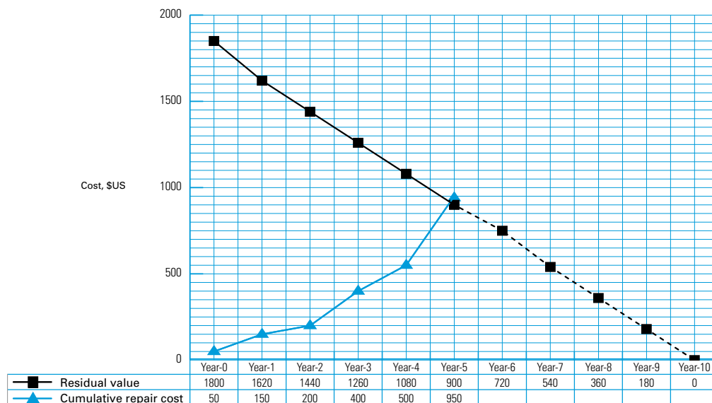
Figure 1.3: Example of equipment replacement point Chart for decision making : repair vs replace
