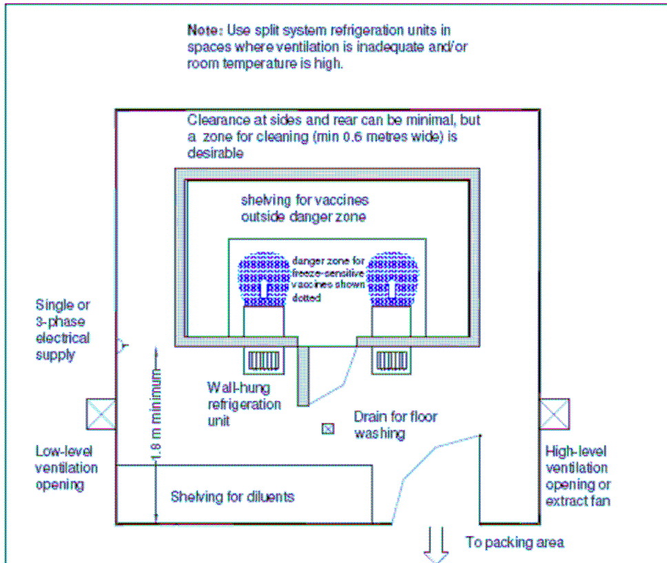
Plan of typical cold room installation
